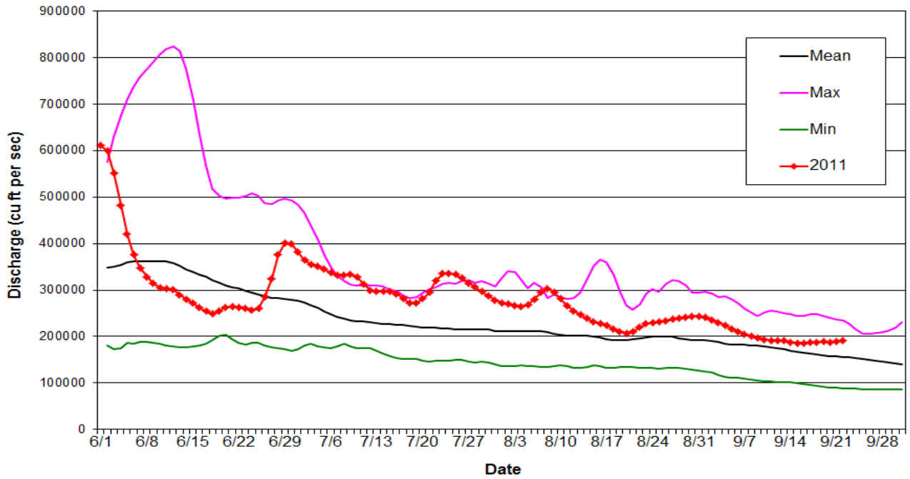
2011 Yukon River Discharge at Rapids (1977-2010 stats) Rapids Research Center
