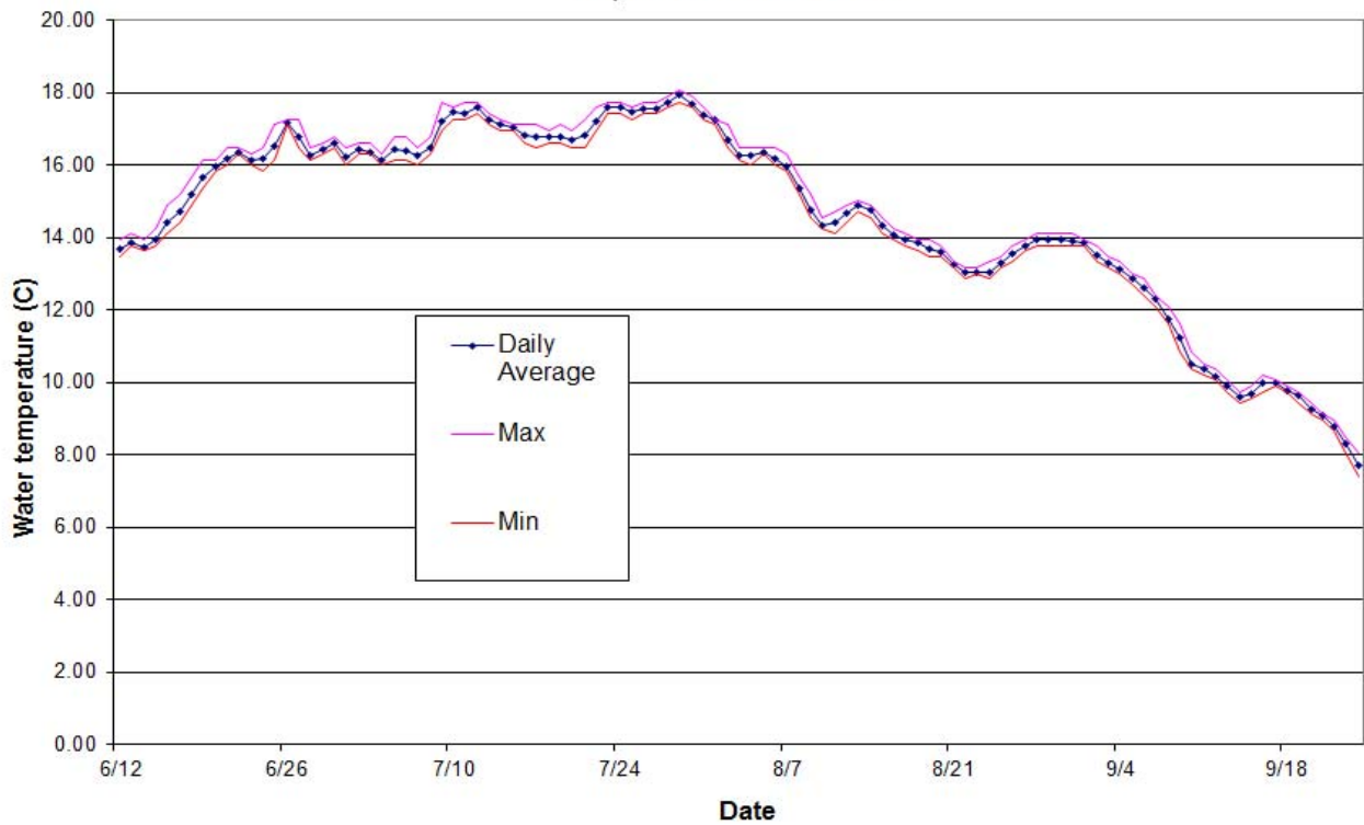
Daily water temperature from Rapids fish wheel site, 2011 Rapids Research Center
