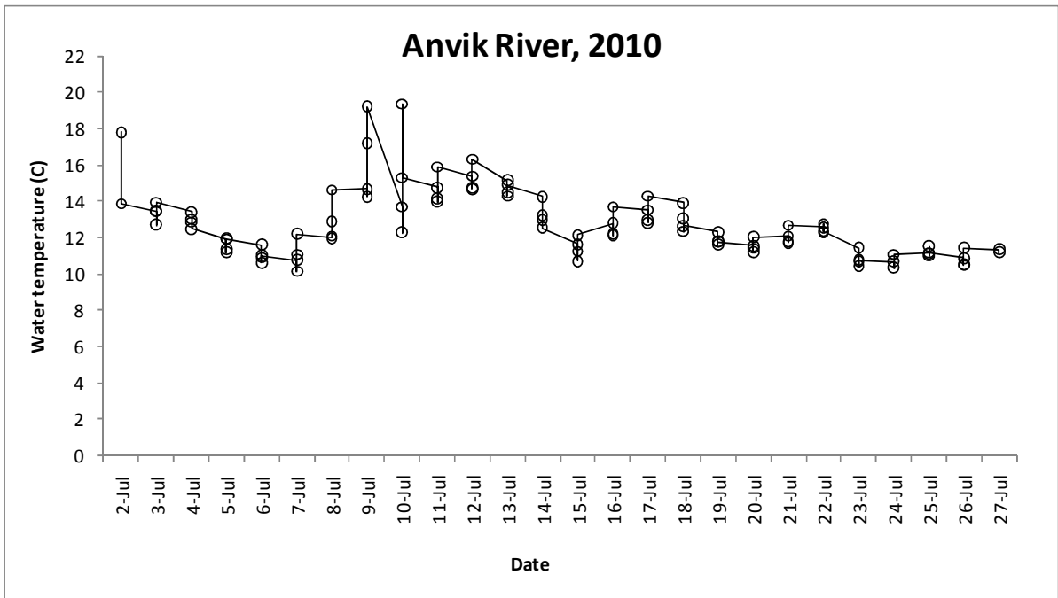
Figure 3.—Water temperature for the Anvik River, 2010. Data was collected every six hours at the sonar site.
