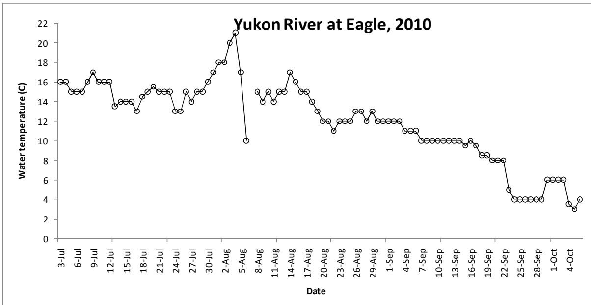
Figure 2.—Mean daily water temperature at Eagle, Alaska, during the 2010 season. Data was collected every four hours at the sonar site.
