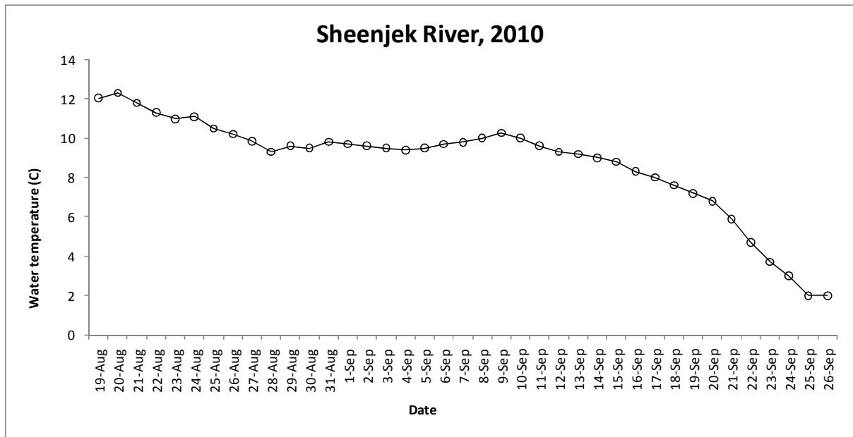
Figure 4.—Mean daily temperature for the Sheenjek River, 2010. Data was collected every four hours at the sonar site.
