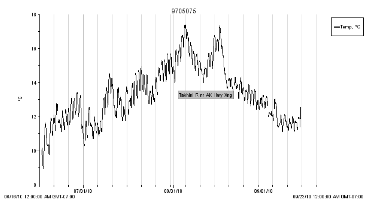
Figure 7.—Water temperature from Takhini River, a tributary to the Yukon River, in the Yukon Territory.
