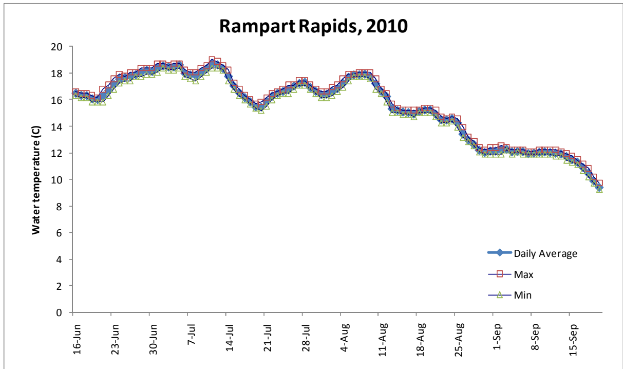
Figure 5.—Mean daily water temperature compared to maximum and minimum taken at Rampart Rapids fish wheel project, 2010.
