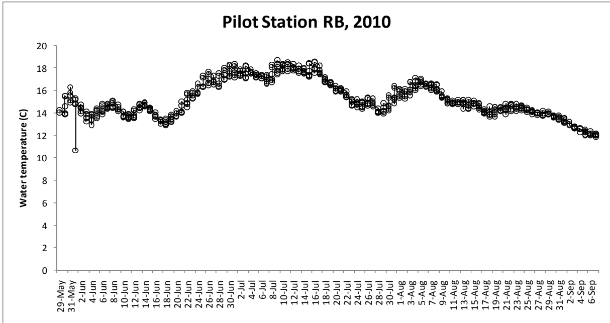
Figure 1.—Water temperature at Pilot Station, Alaska, during the 2010 season. Data was collected every four hours at the right bank sonar site.
