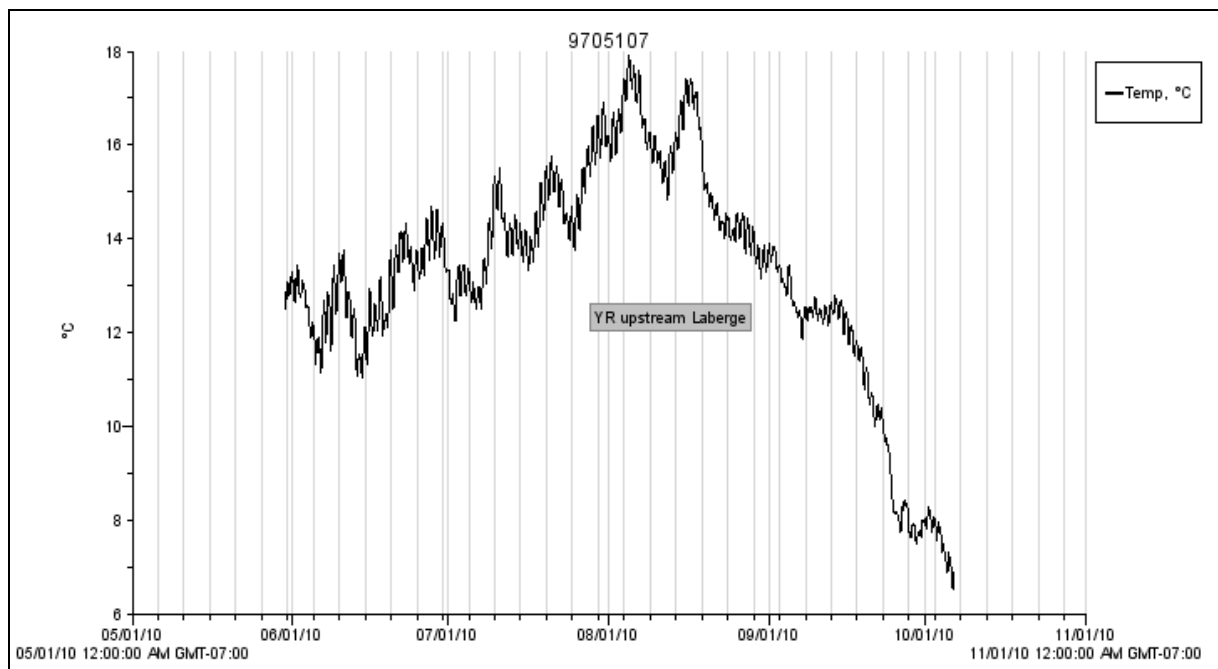
Figure 6.—Water temperature from directly upstream of Lake Laberge within the Yukon River mainstem, Yukon Territory, 2010.
