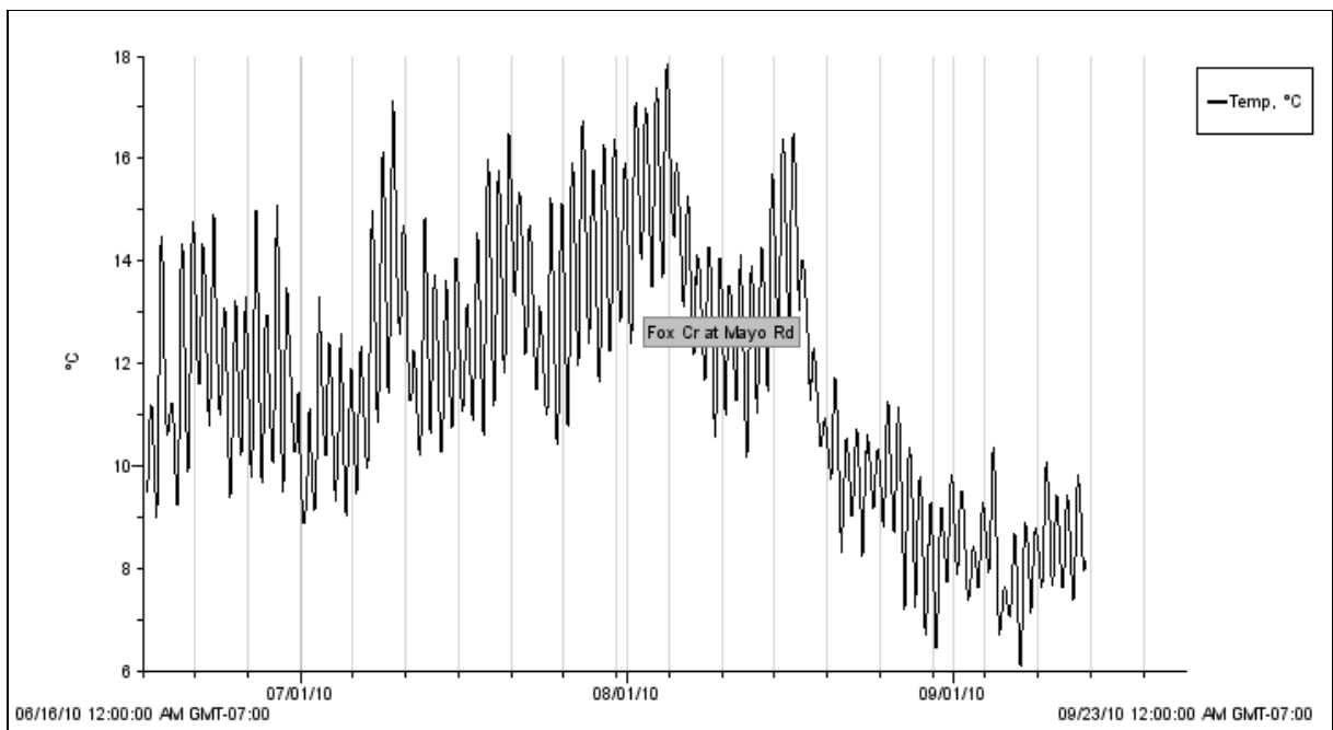
Figure 8.—Water temperature from Fox Creek, a tributary to the Yukon River, Yukon Territory.
