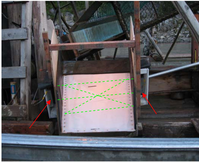
Infrared transmitter / receiver placement (red), and direction of beams across chute (green).
