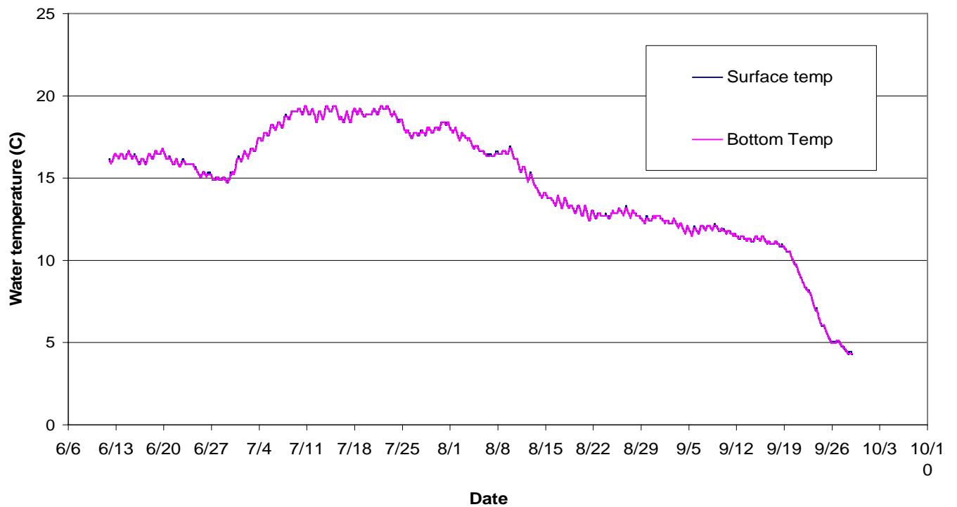
Hourly surface (1 m depth) and bottom (4.3 m depth) water temperature, Rapids video fish wheel, 2009. Evidence of complete mixing at site. Rapids Research Center
