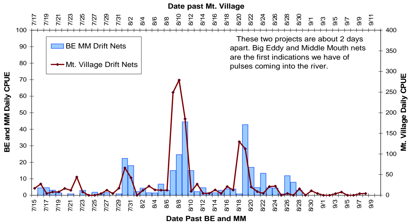
BE and MM Drift Nets Compared to Mt. Village Drift Nets Fall Chum 2009, Rapids Research Center
