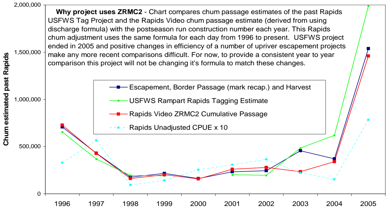
1996 to 2005 Upper Yukon Fall Chum Escapement Projects, Border Passage and Harvest Combined and Compared to Rapids Video, Discharge Adjusted CPUE (ZRMC2) and USFWS Rampart Rapids Tagging Estimate (Rapids Research Center)
